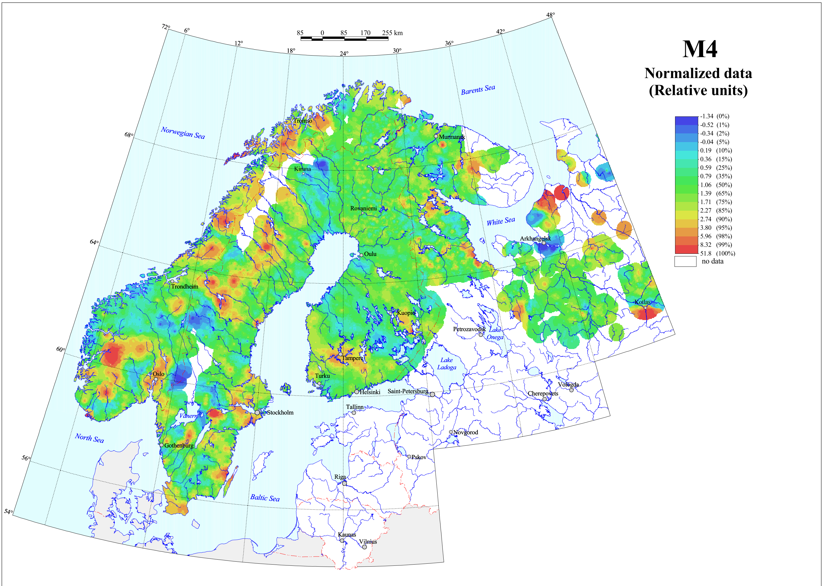
M4 (Mo, Pb, Zn) in Till, Grain Size <0.06 mm
